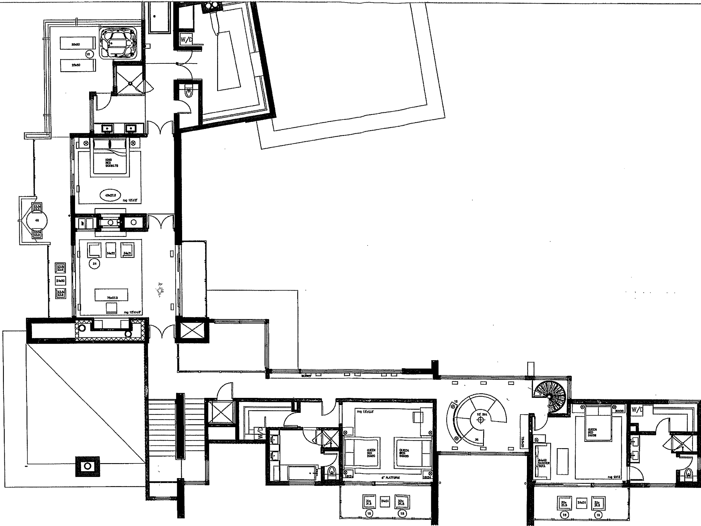
1 FLOORPLAN FP-3 UPPER LEVEL
